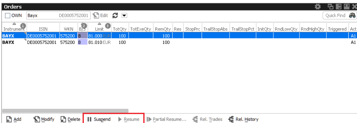
Fig. 58: Screenshot of the Orders view showing the Suspend and Resume actions
