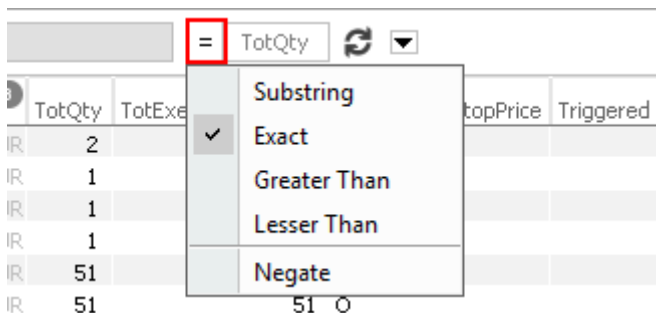
Fig. 23: Filter Restrictions
