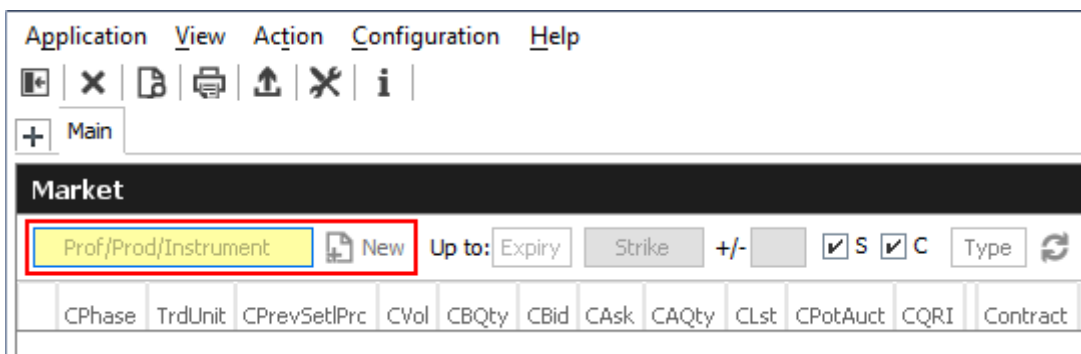
Fig. 35: Profile/Product Selector
