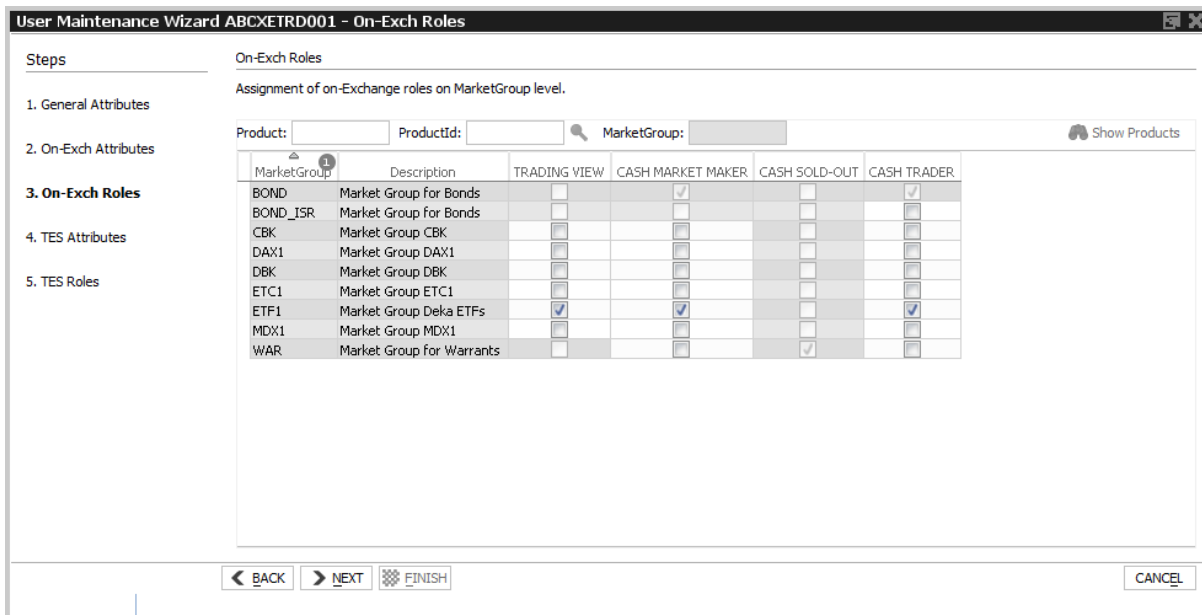
Fig. 102: Screenshot of the User Maintenance Wizard showing the entitlement roles on the On-Exch Roles tab
