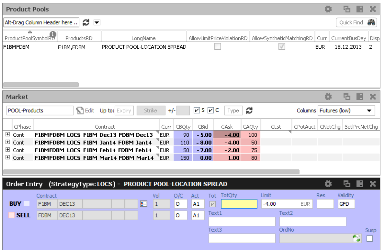
Fig. 130: Screenshot showing the Product Pools view.
