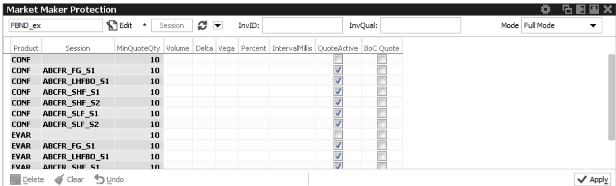
Fig. 76: Screenshot of the Market Maker Protection view
