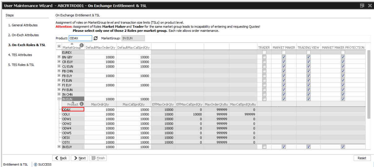
Fig. 151: Screenshot of the User Maintenance Wizard showing the On Exchange Entitlement & TSL tab
