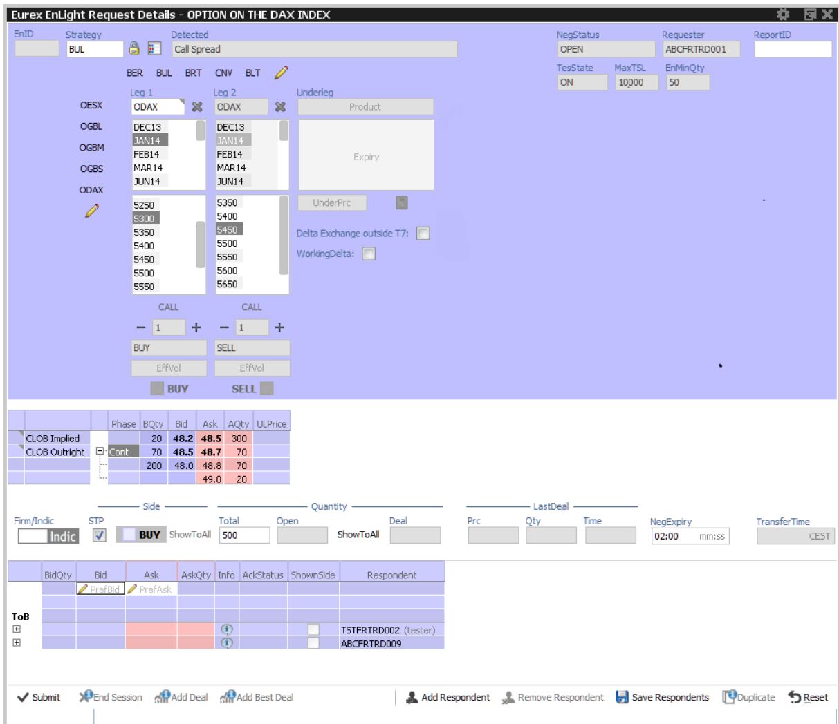
Fig. 102: Screenshot of the Eurex EnLight Request Details view showing a BUL strategy and new CLOB data display
