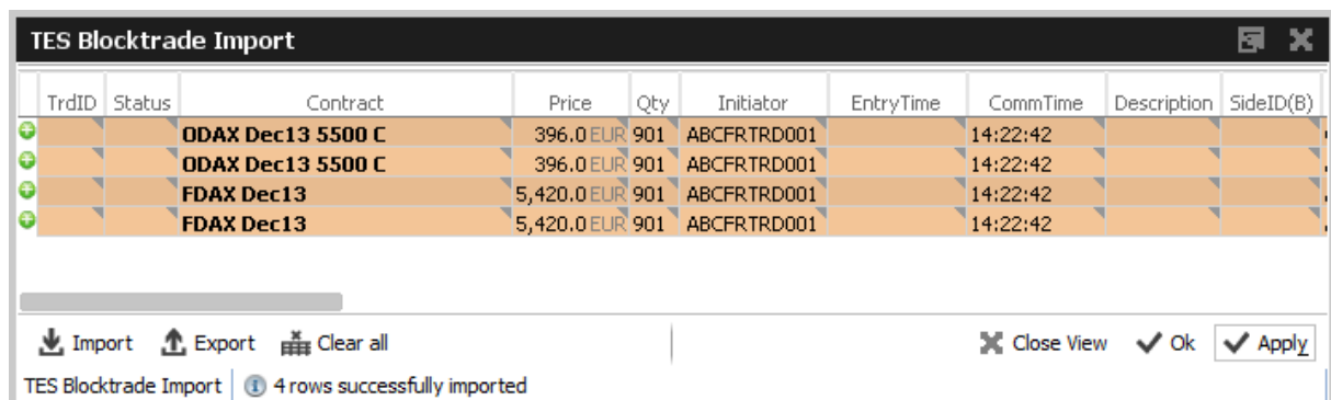
Fig. 80: Screenshot of the Block Trade Service Bulk Load view
