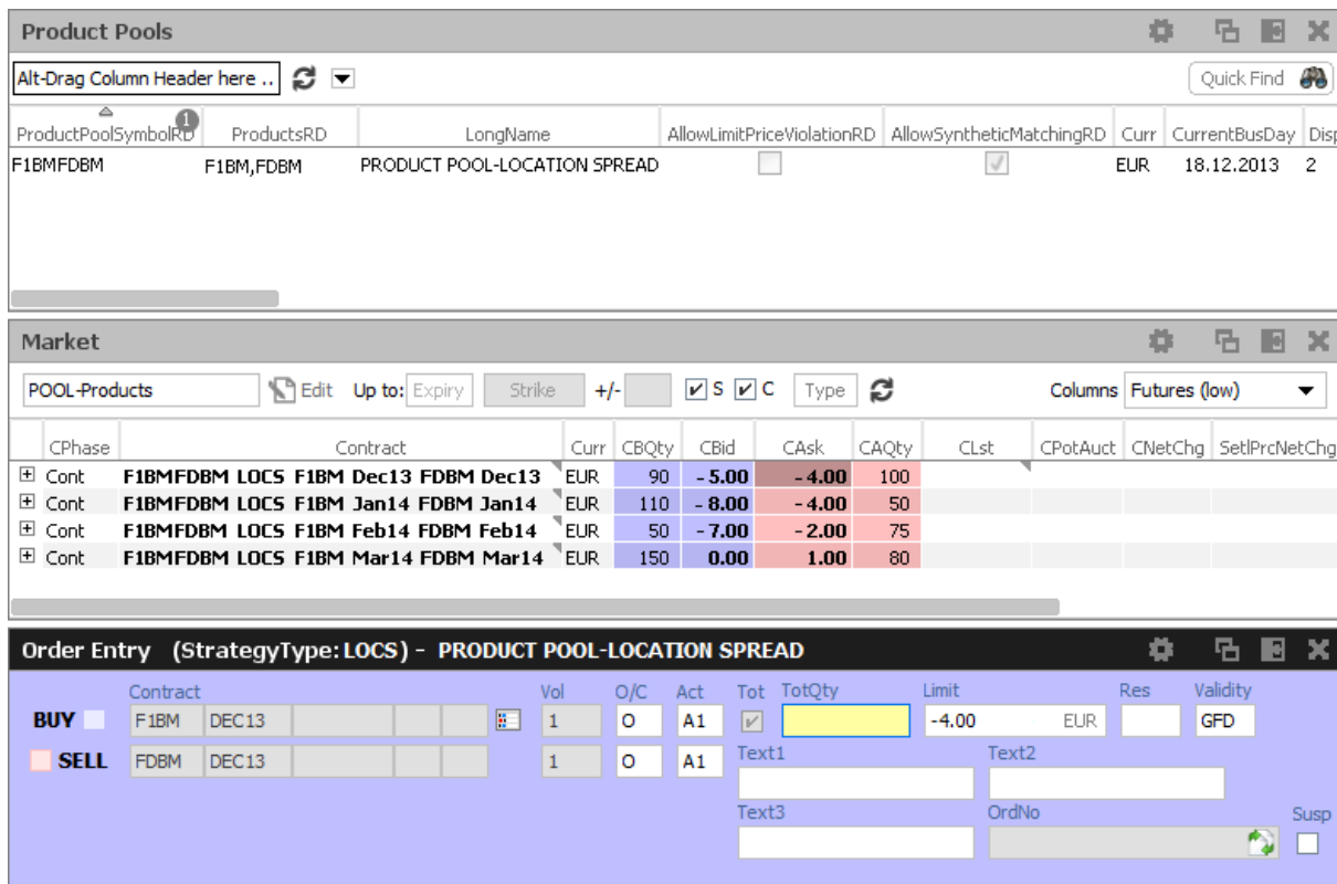
Fig. 133: Screenshot showing the Product Pools view.
