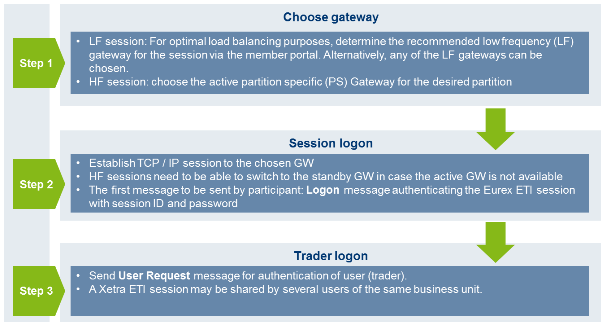
Figure 17: Xetra ETI session logon process
